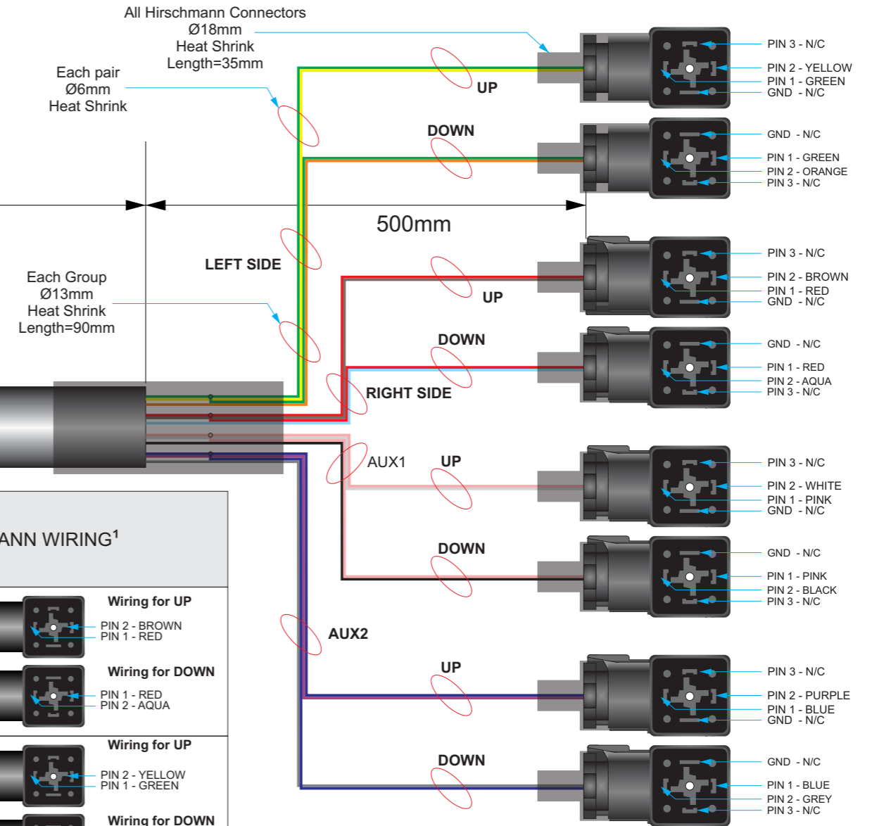
8 x Hirschmann Connectors (P.CONN.043)
